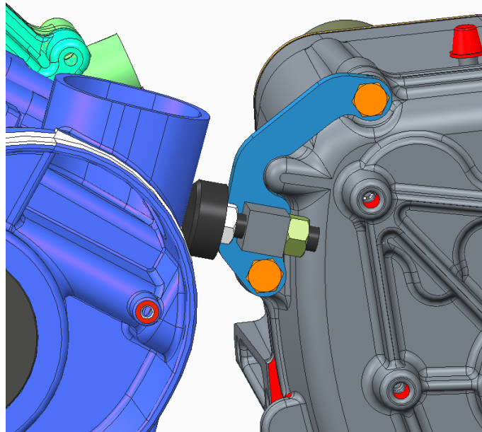
MODEL OF TORQUE STOP INSTALLATION WITH CLUTCH HOUSING BACK REMOVED
